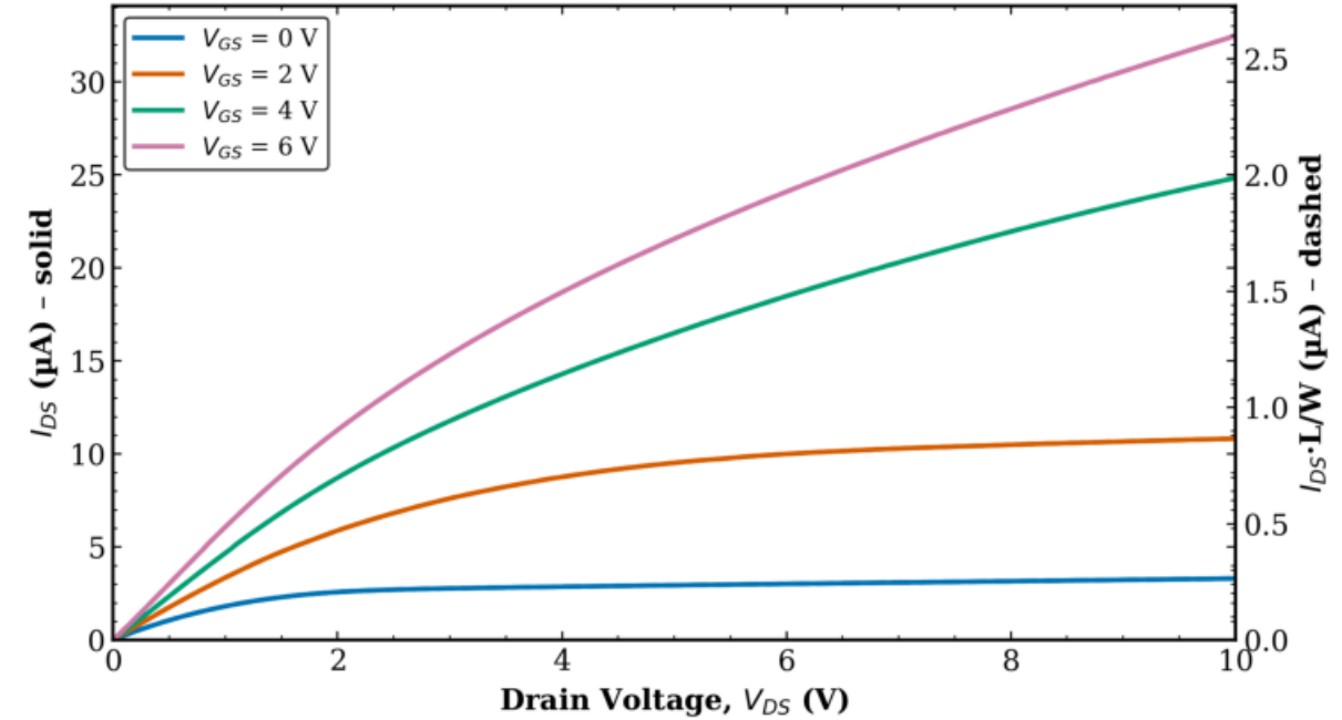
TFT2 Combined (Tr. 1 & 2) L = 40 \mu\text{m} , W = 500 \mu\text{m}
