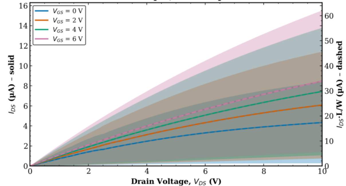
TFT2 Combined (Tr. 1 & 2) L = 40 \mu\text{m} , W = 10 \mu\text{m}
