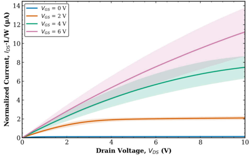
TFT2 Combined (Tr. 1 & 2) L = 160 \mu\text{m} , W = 10 \mu\text{m} (normalized)
