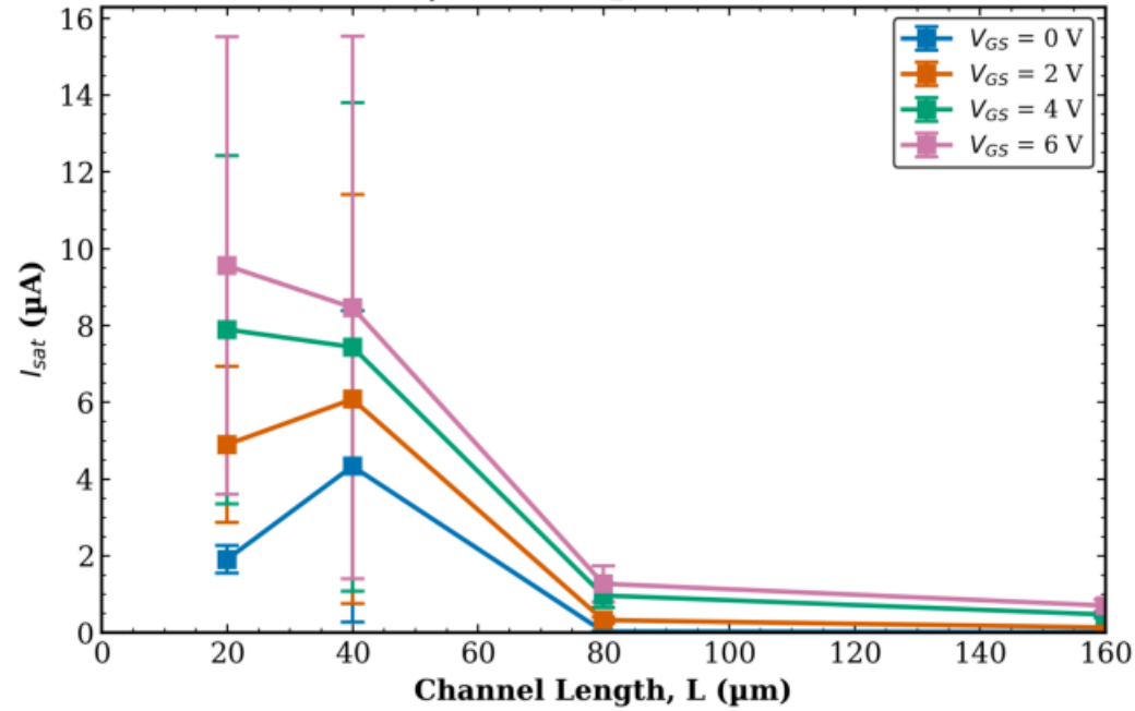
TFT2 Combined (Tr. 1 & 2) I_{sat} vs L | W = 10 \mu\text{m} (mean \pm std)
