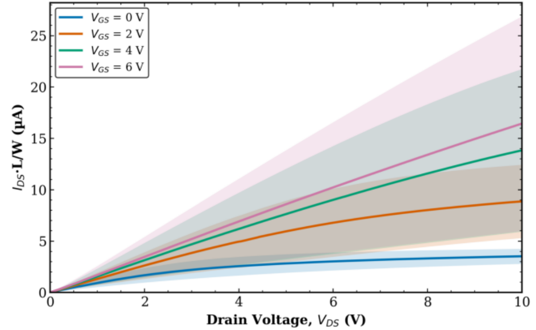
TFT2 Combined (Tr. 1 & 2) L = 20 \mu\text{m} - avg over all W (mean \pm std)
