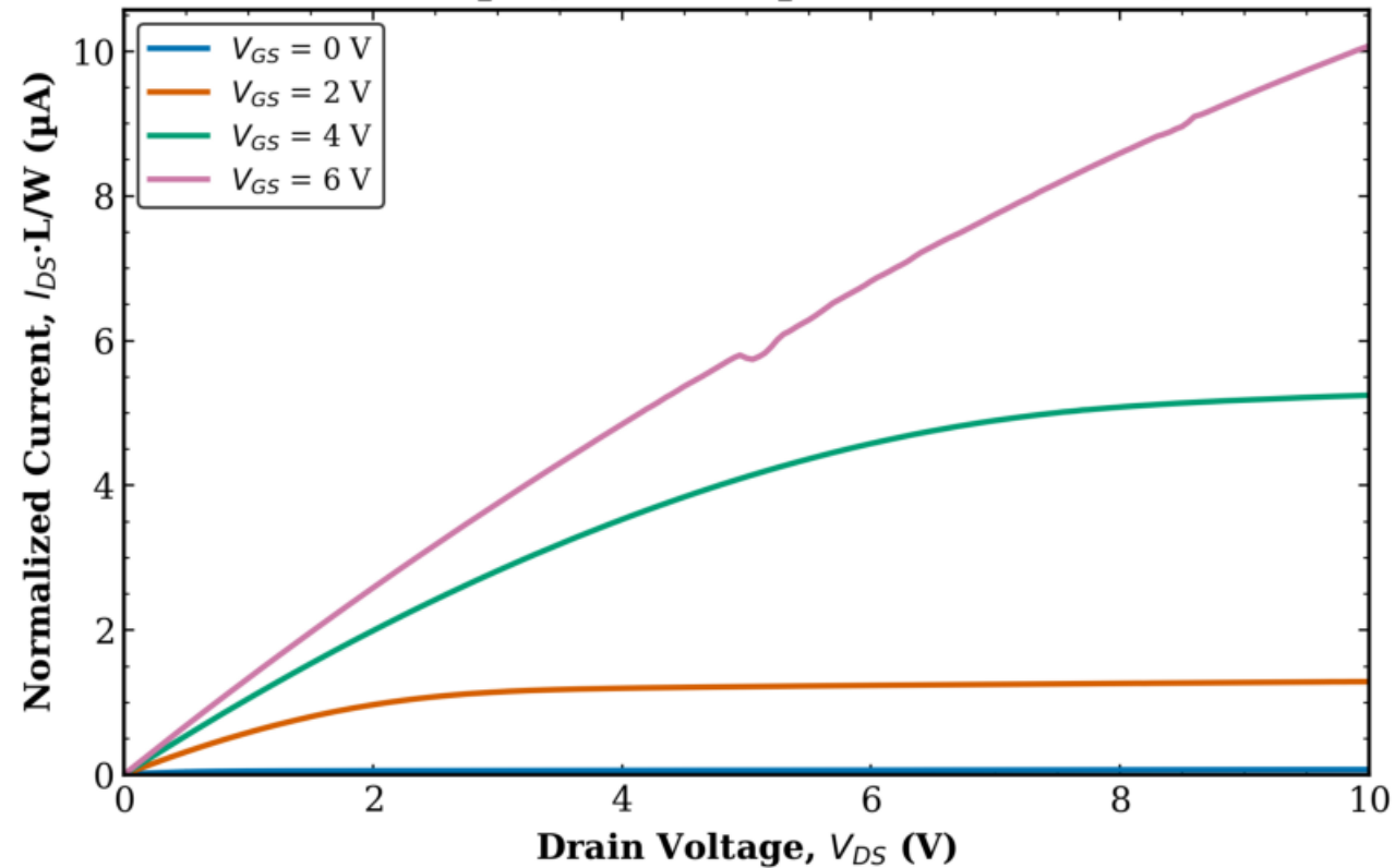
TFT2 Combined (Tr. 1 & 2) L = 80 \mu\text{m} , W = 50 \mu\text{m} (normalized)
