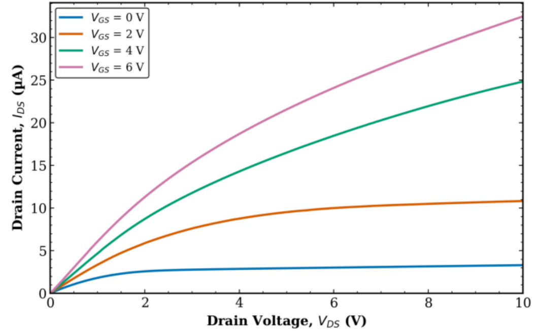
TFT2 Combined (Tr. 1 & 2) L = 40 \mu\text{m} , W = 500 \mu\text{m}
