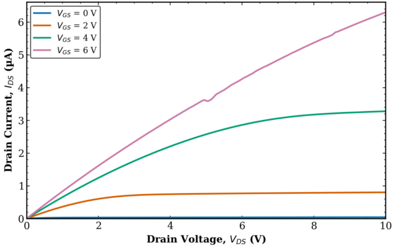
TFT2 Combined (Tr. 1 & 2) L = 80 \mu\text{m} , W = 50 \mu\text{m}
