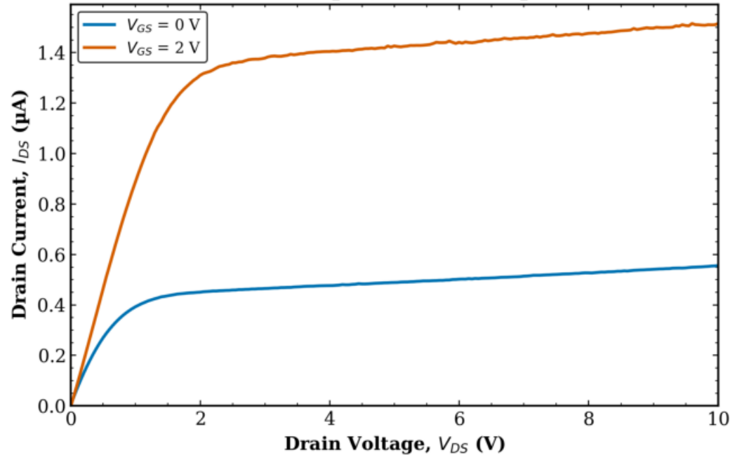
TFT2 Combined (Tr. 1 & 2) L = 160 \mu\text{m} , W = 1000 \mu\text{m}
