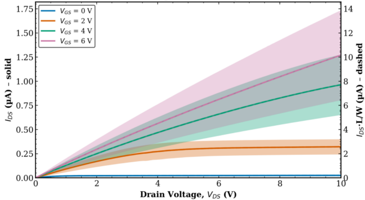
TFT2 Combined (Tr. 1 & 2) L = 80 \mu\text{m} , W = 10 \mu\text{m}
