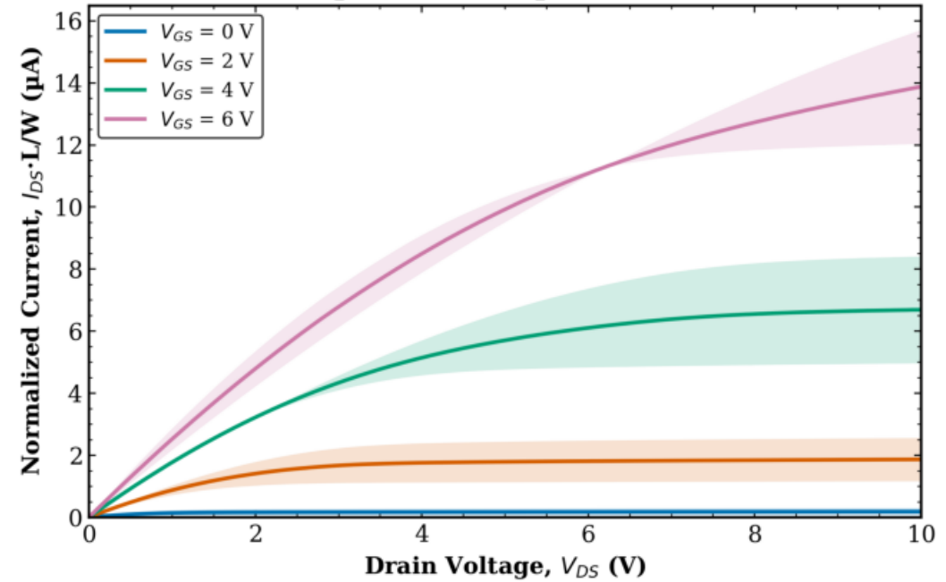
TFT2 Combined (Tr. 1 & 2) L = 160 \mu\text{m} , W = 50 \mu\text{m} (normalized)
