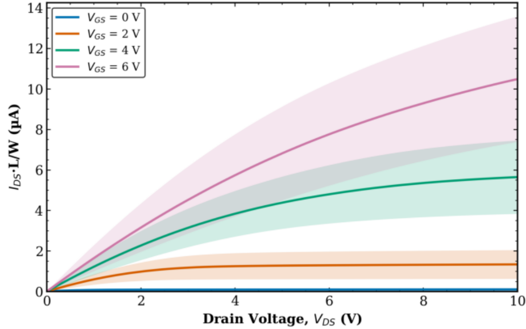
TFT2 Combined (Tr. 1 & 2) L = 160 \mu\text{m} - avg over all W (mean \pm std)
