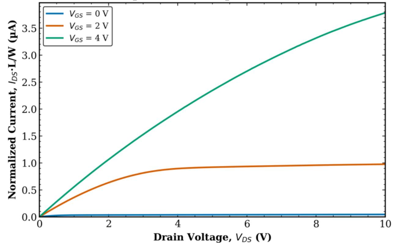
TFT2 Combined (Tr. 1 & 2) L = 80 \mu\text{m} , W = 500 \mu\text{m} (normalized)
