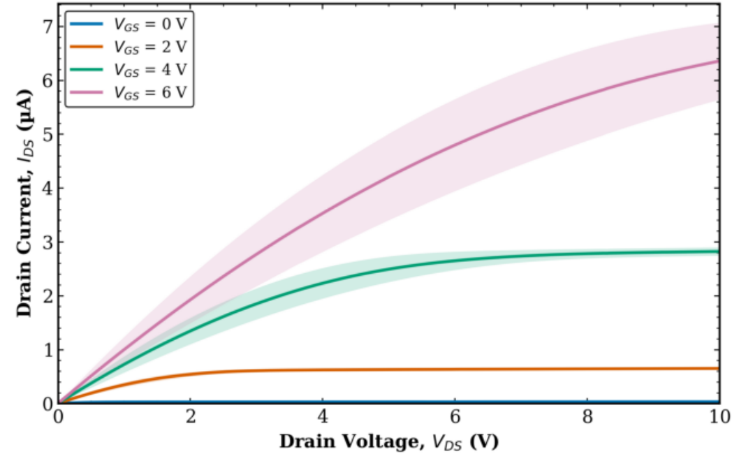
TFT2 Combined (Tr. 1 & 2) L = 160 \mu\text{m} , W = 100 \mu\text{m}
