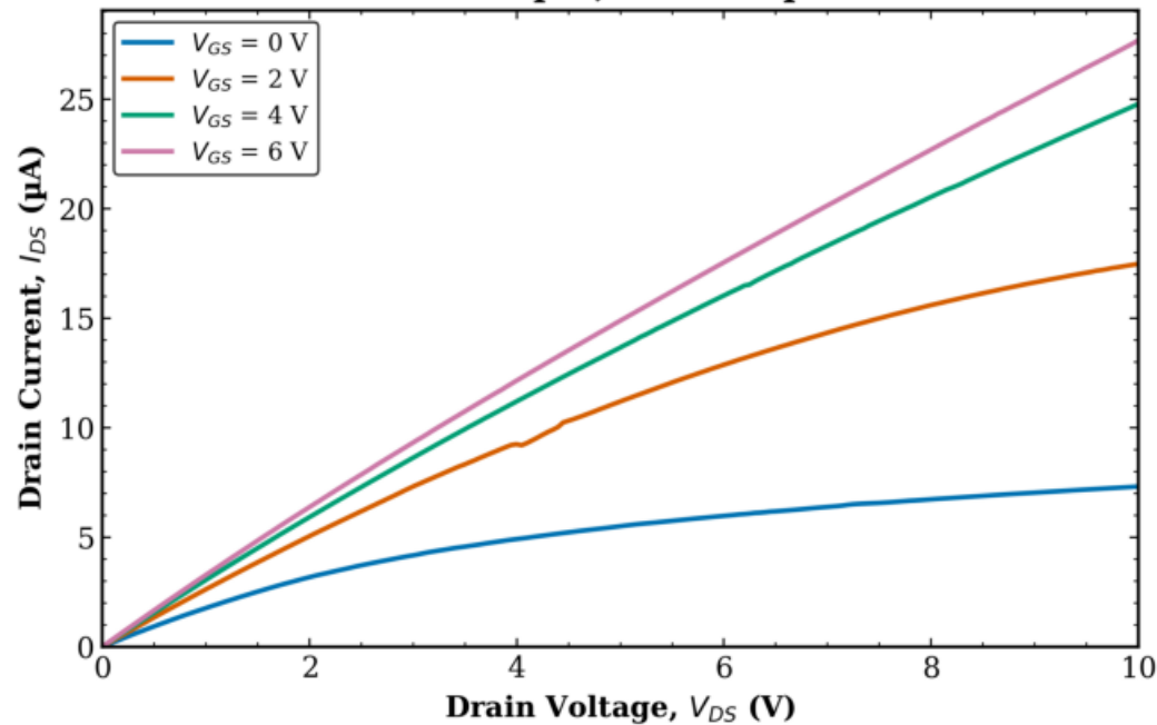
TFT2 Combined (Tr. 1 & 2) L = 20 \mu\text{m} , W = 50 \mu\text{m}
