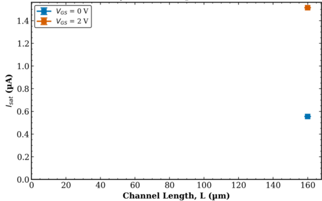
TFT2 Combined (Tr. 1 & 2) I_{sat} vs L | W = 1000 μm (mean \pm std)
