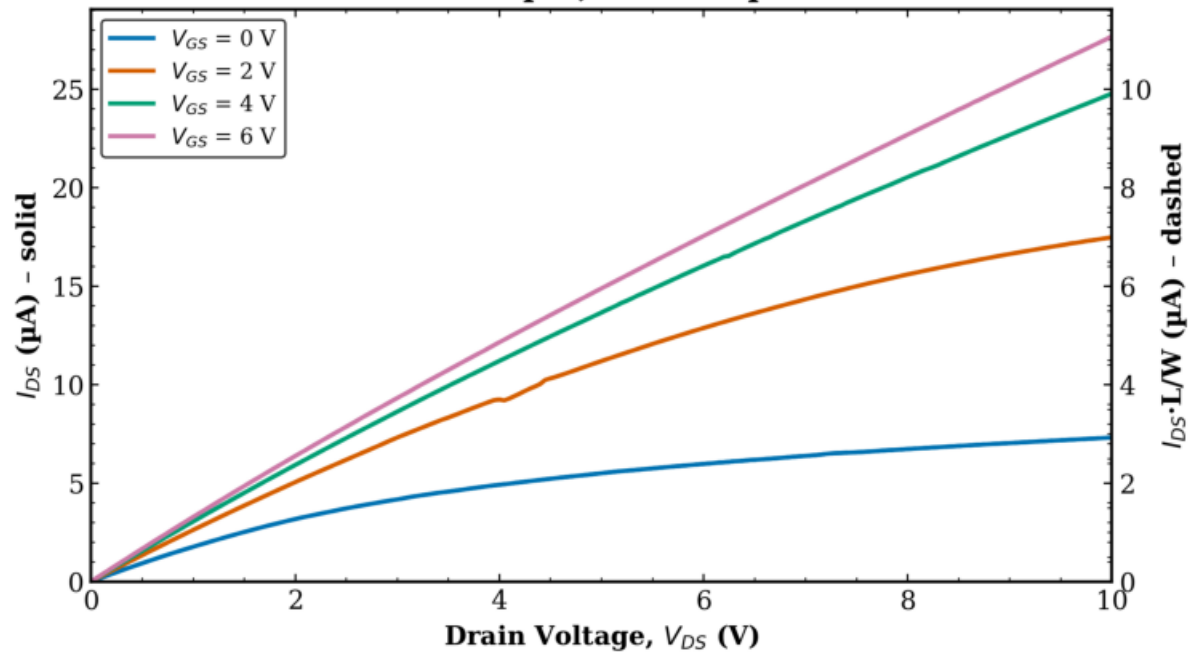
TFT2 Combined (Tr. 1 & 2) L = 20 \mu\text{m} , W = 50 \mu\text{m}
