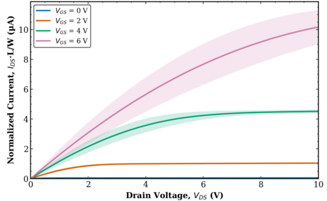
TFT2 Combined (Tr. 1 & 2) L = 160 \mu\text{m} , W = 100 \mu\text{m} (normalized)
