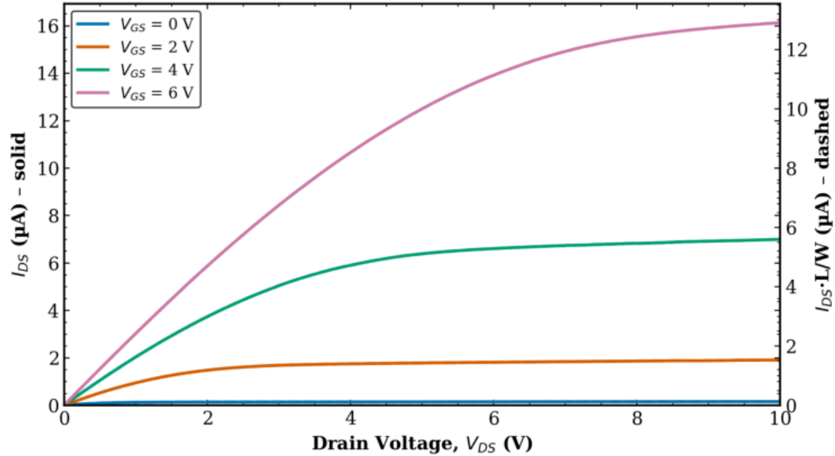
TFT2 Combined (Tr. 1 & 2) L = 40 \mu\text{m} , W = 50 \mu\text{m}
