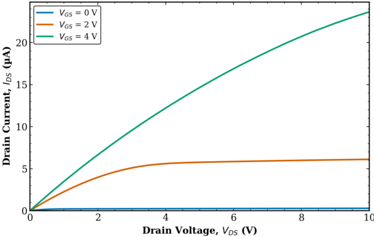
TFT2 Combined (Tr. 1 & 2) L = 80 \mu\text{m} , W = 500 \mu\text{m}
