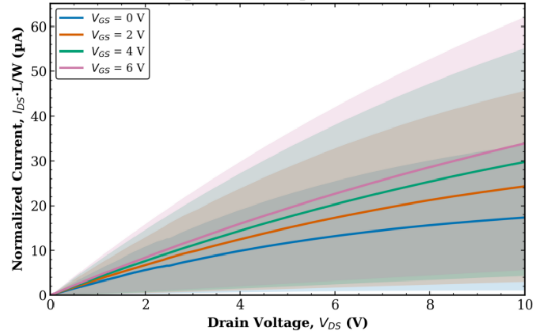
TFT2 Combined (Tr. 1 & 2) L = 40 \mu\text{m} , W = 10 \mu\text{m} (normalized)
