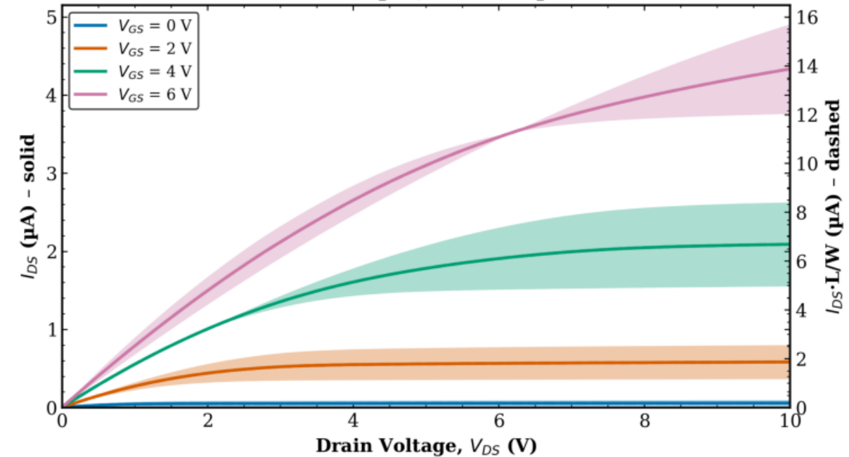
TFT2 Combined (Tr. 1 & 2) L = 160 \mu\text{m} , W = 50 \mu\text{m}
