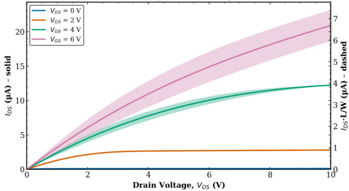
TFT2 Combined (Tr. 1 & 2) L = 160 \mu\text{m} , W = 500 \mu\text{m}
