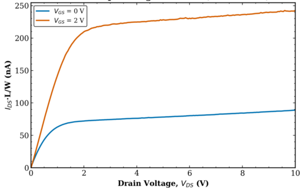
TFT2 Combined (Tr. 1 & 2) W = 1000 \mu\text{m} - avg over all L (mean \pm std)
