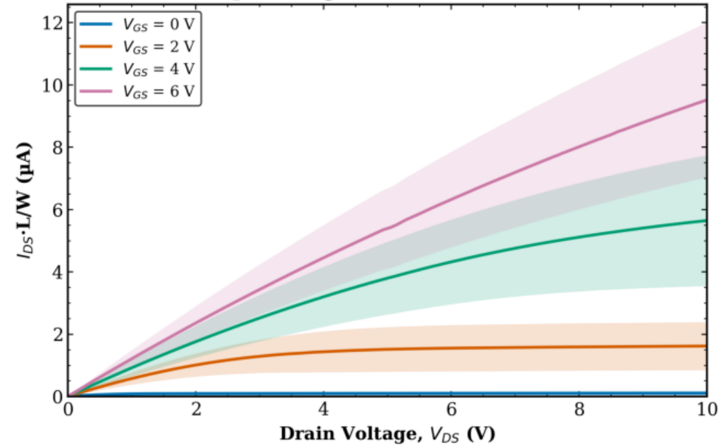
TFT2 Combined (Tr. 1 & 2) L = 80 \mu\text{m} - avg over all W (mean \pm std)
