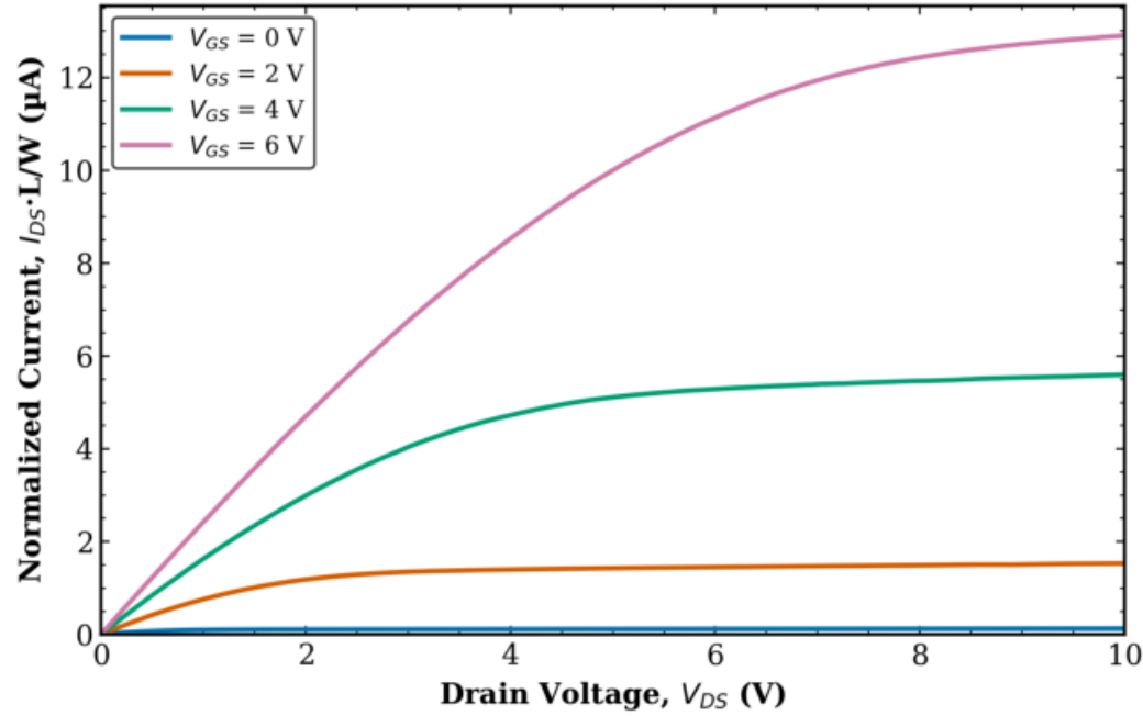
TFT2 Combined (Tr. 1 & 2) L = 40 \mu\text{m} , W = 50 \mu\text{m} (normalized)
