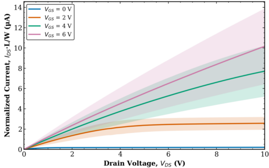
TFT2 Combined (Tr. 1 & 2) L = 80 \mu\text{m} , W = 10 \mu\text{m} (normalized)
