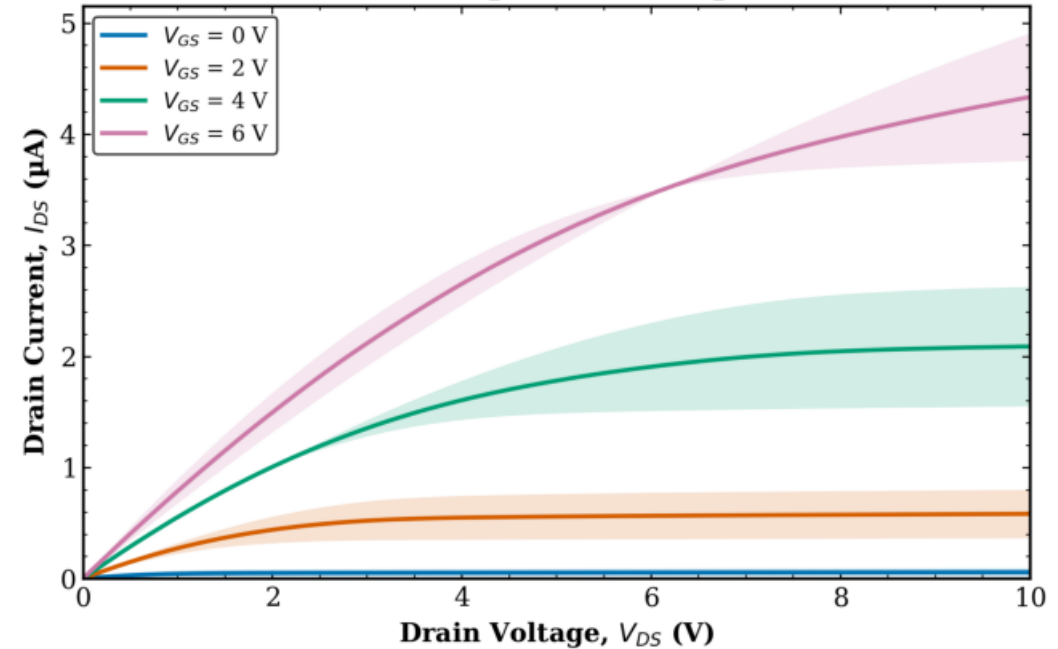
TFT2 Combined (Tr. 1 & 2) L = 160 \mu\text{m} , W = 50 \mu\text{m}
