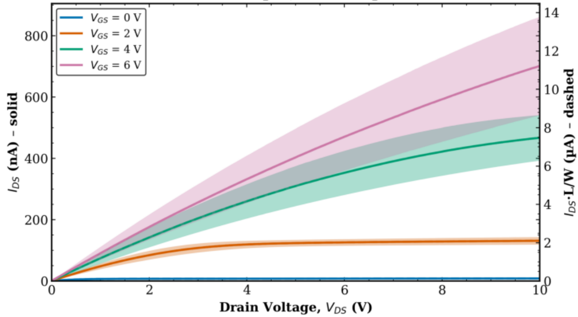
TFT2 Combined (Tr. 1 & 2) L = 160 \mu\text{m} , W = 10 \mu\text{m}
