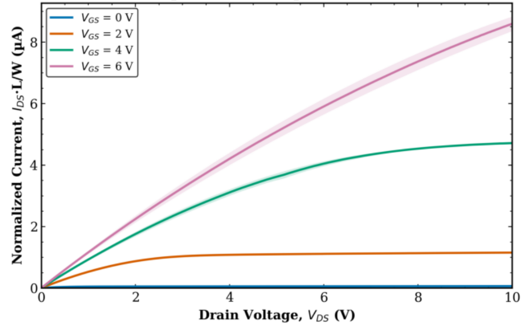
TFT2 Combined (Tr. 1 & 2) L = 80 \mu\text{m} , W = 100 \mu\text{m} (normalized)
