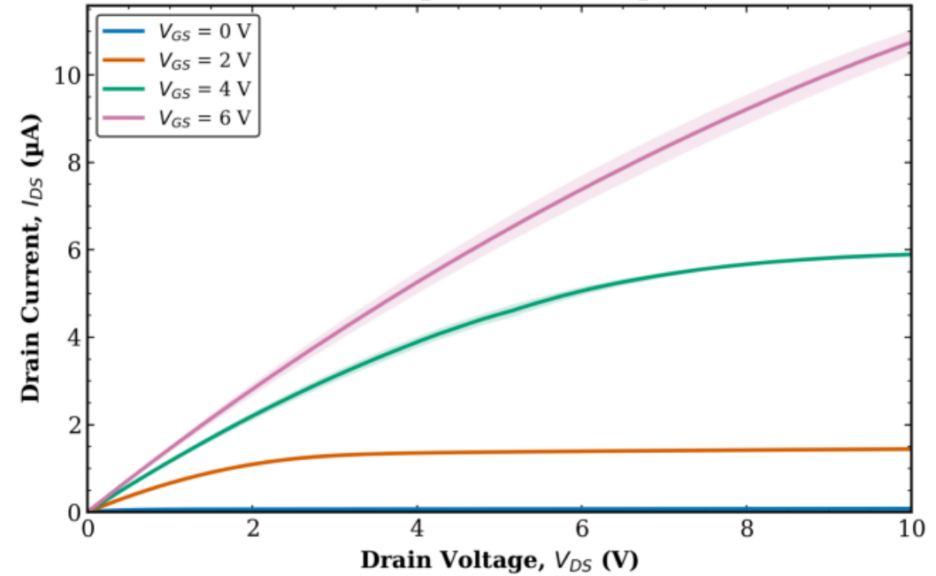
TFT2 Combined (Tr. 1 & 2) L = 80 \mu\text{m} , W = 100 \mu\text{m}
