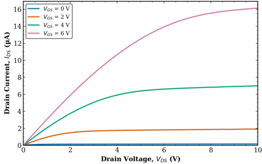
TFT2 Combined (Tr. 1 & 2) L = 40 \mu\text{m} , W = 50 \mu\text{m}
