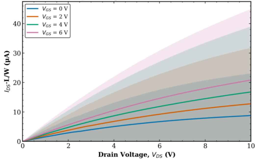
TFT2 Combined (Tr. 1 & 2) L = 40 \mu\text{m} - avg over all W (mean \pm std)
