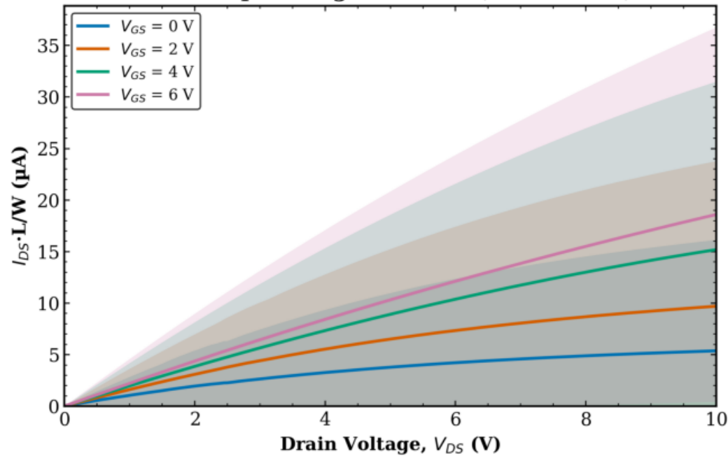
TFT2 Combined (Tr. 1 & 2) W = 10 \mu\text{m} - avg over all L (mean \pm std)
