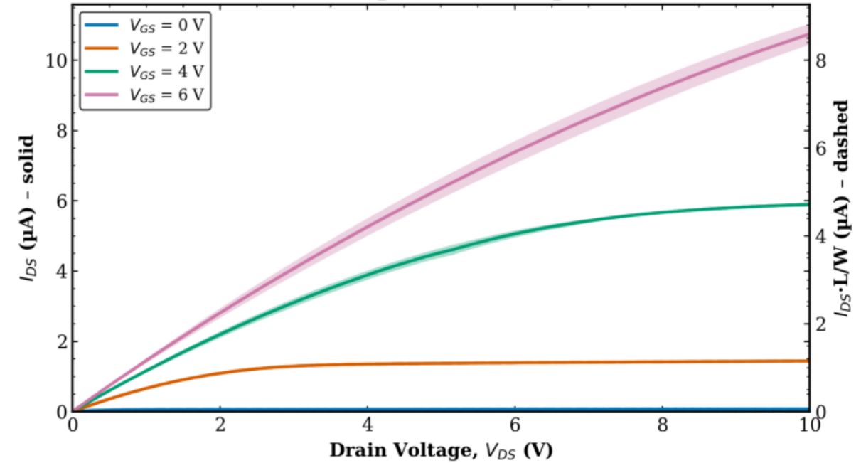
TFT2 Combined (Tr. 1 & 2) L = 80 \mu\text{m} , W = 100 \mu\text{m}
