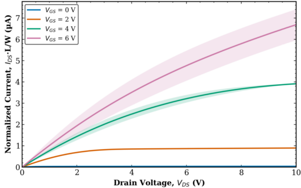
TFT2 Combined (Tr. 1 & 2) L = 160 \mu\text{m} , W = 500 \mu\text{m} (normalized)
