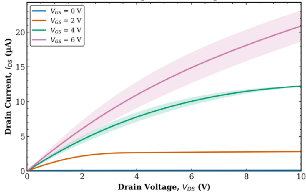
TFT2 Combined (Tr. 1 & 2) L = 160 \mu\text{m} , W = 500 \mu\text{m}
