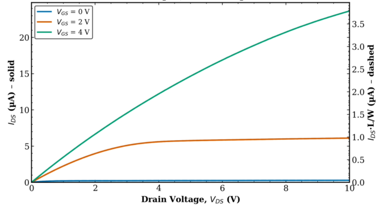
TFT2 Combined (Tr. 1 & 2) L = 80 \mu\text{m} , W = 500 \mu\text{m}
