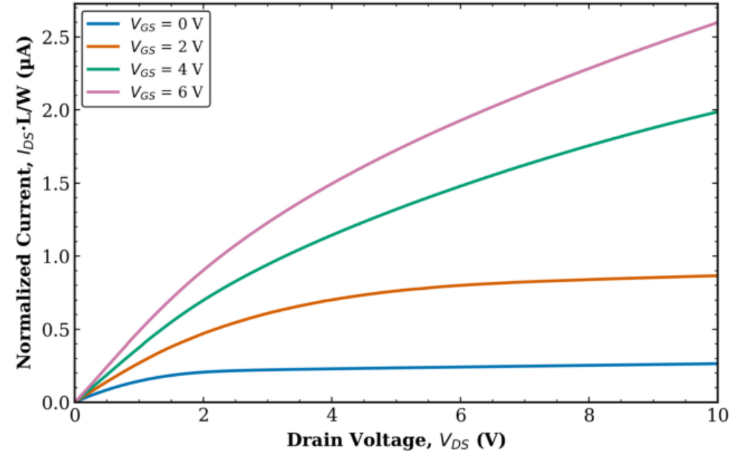
TFT2 Combined (Tr. 1 & 2) L = 40 \mu\text{m} , W = 500 \mu\text{m} (normalized)
