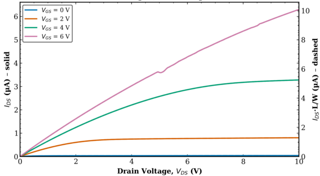
TFT2 Combined (Tr. 1 & 2) L = 80 \mu\text{m} , W = 50 \mu\text{m}
