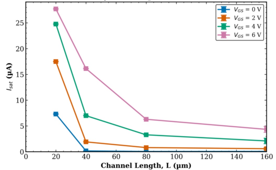
TFT2 Combined (Tr. 1 & 2) I_{sat} vs L | W = 50 μm (mean \pm std)
