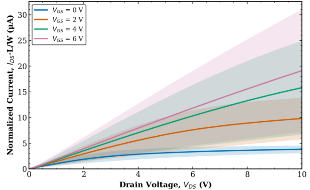
TFT2 Combined (Tr. 1 & 2) L = 20 \mu\text{m} , W = 10 \mu\text{m} (normalized)
