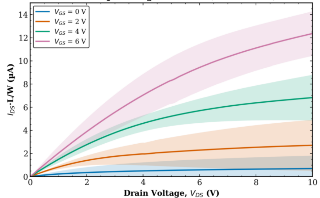
TFT2 Combined (Tr. 1 & 2) W = 50 \mu\text{m} - avg over all L (mean \pm std)
