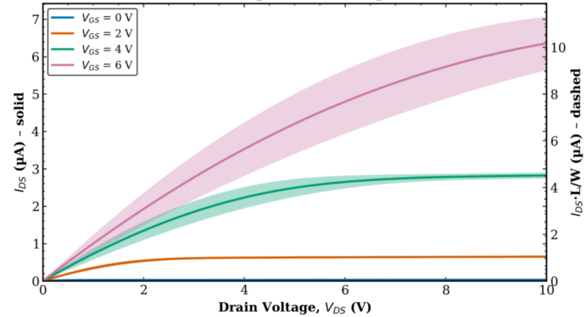
TFT2 Combined (Tr. 1 & 2) L = 160 \mu\text{m} , W = 100 \mu\text{m}
