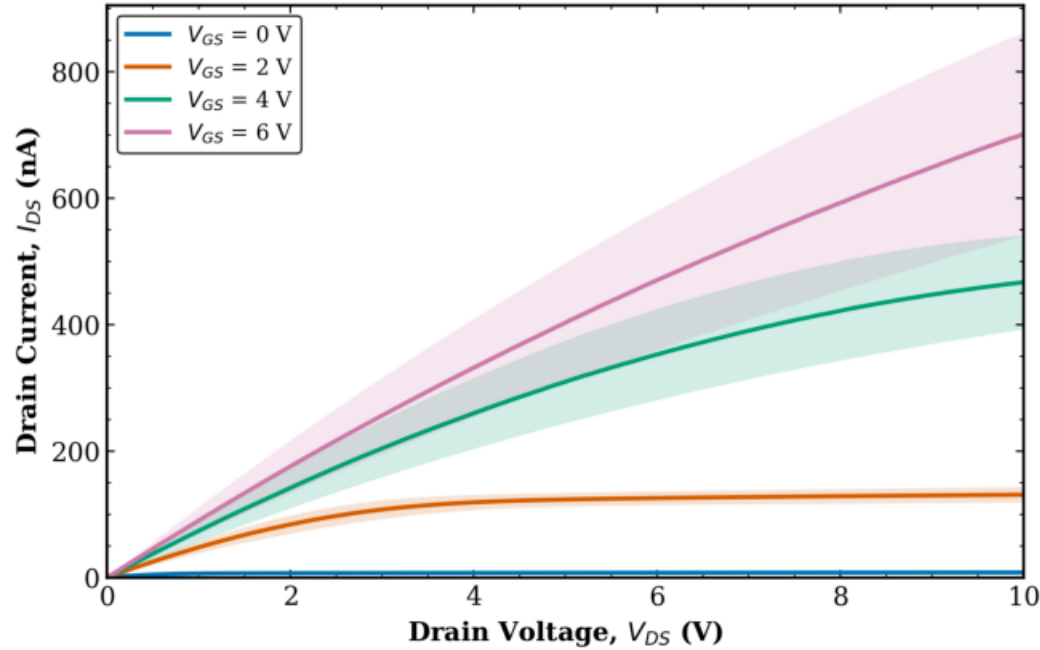
TFT2 Combined (Tr. 1 & 2) L = 160 \mu\text{m} , W = 10 \mu\text{m}
