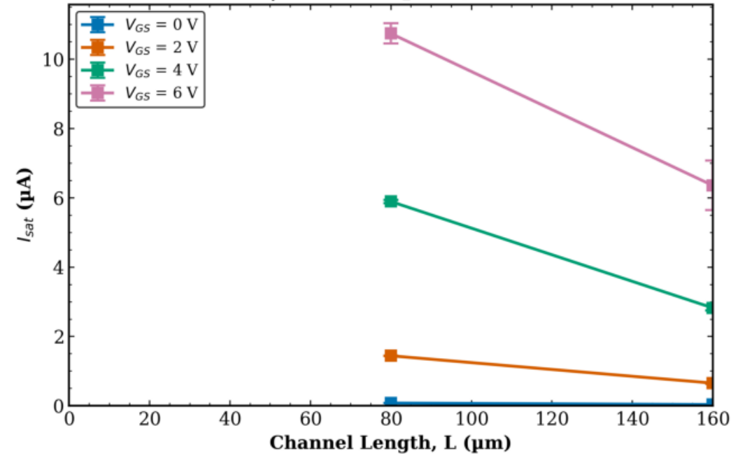
TFT2 Combined (Tr. 1 & 2) I_{sat} vs L | W = 100 μm (mean \pm std)
