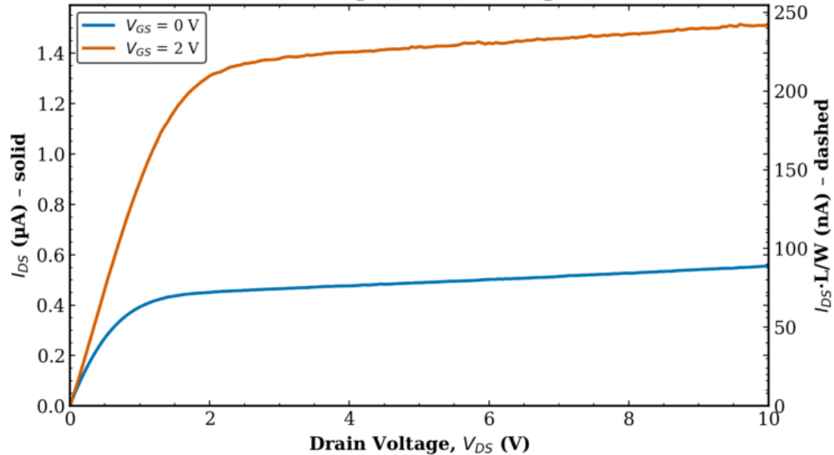
TFT2 Combined (Tr. 1 & 2) L = 160 \mu\text{m} , W = 1000 \mu\text{m}
