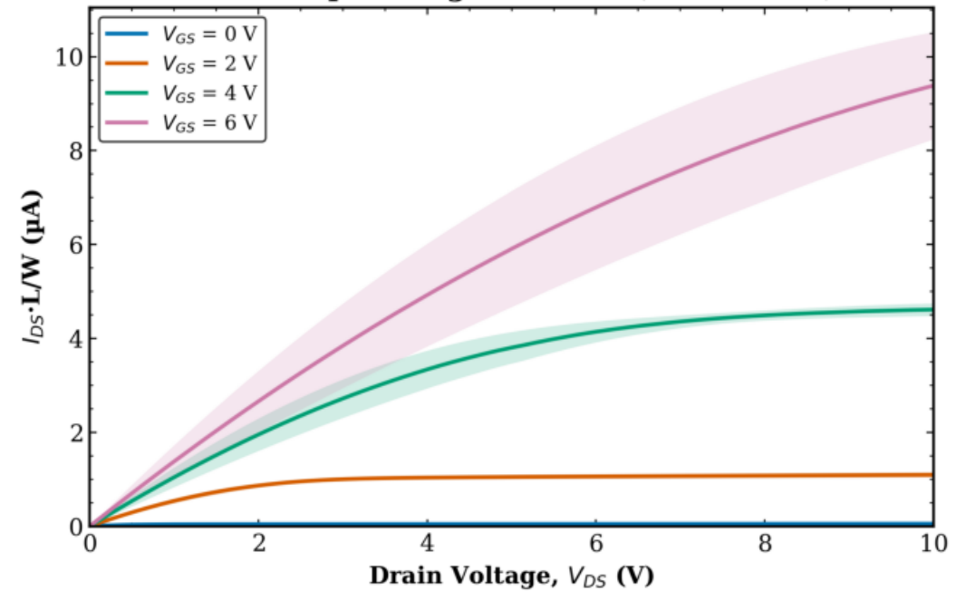
TFT2 Combined (Tr. 1 & 2) W = 100 \mu\text{m} - avg over all L (mean \pm std)
