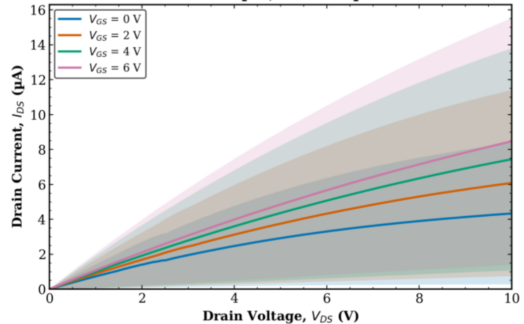
TFT2 Combined (Tr. 1 & 2) L = 40 \mu\text{m} , W = 10 \mu\text{m}
