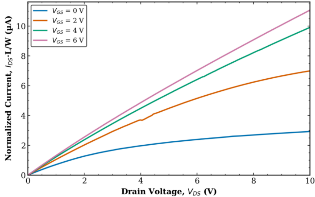
TFT2 Combined (Tr. 1 & 2) L = 20 \mu\text{m} , W = 50 \mu\text{m} (normalized)
